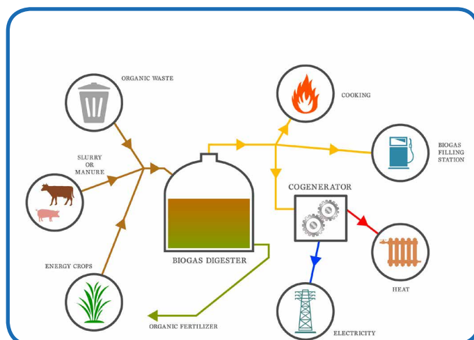
Fig. 2: Schematic of a typical AD Biogas plant showing the various feedstock used to produce green energy in the form of heat, biomethane and electricity.
